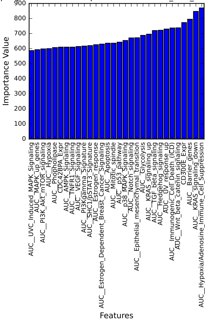
Top LightGBM Feature Importance MolFormer_Feat_Var_random
