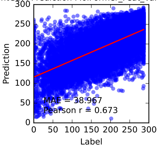
LightGBM Prediction MolFormer_Feat_Var_random
