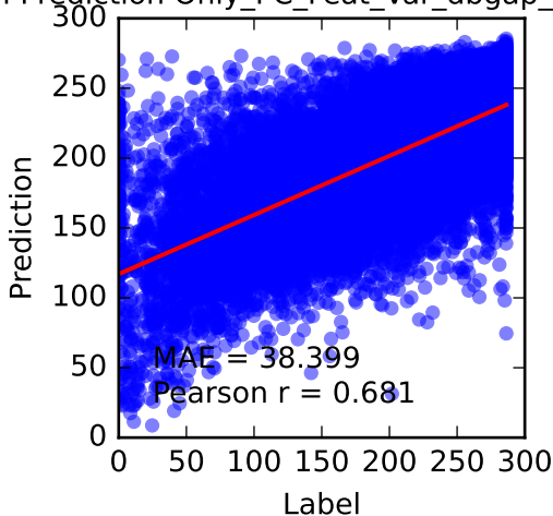
LightGBM Prediction Only_PC_Feat_Var_dbgap_rnaseq_sample
