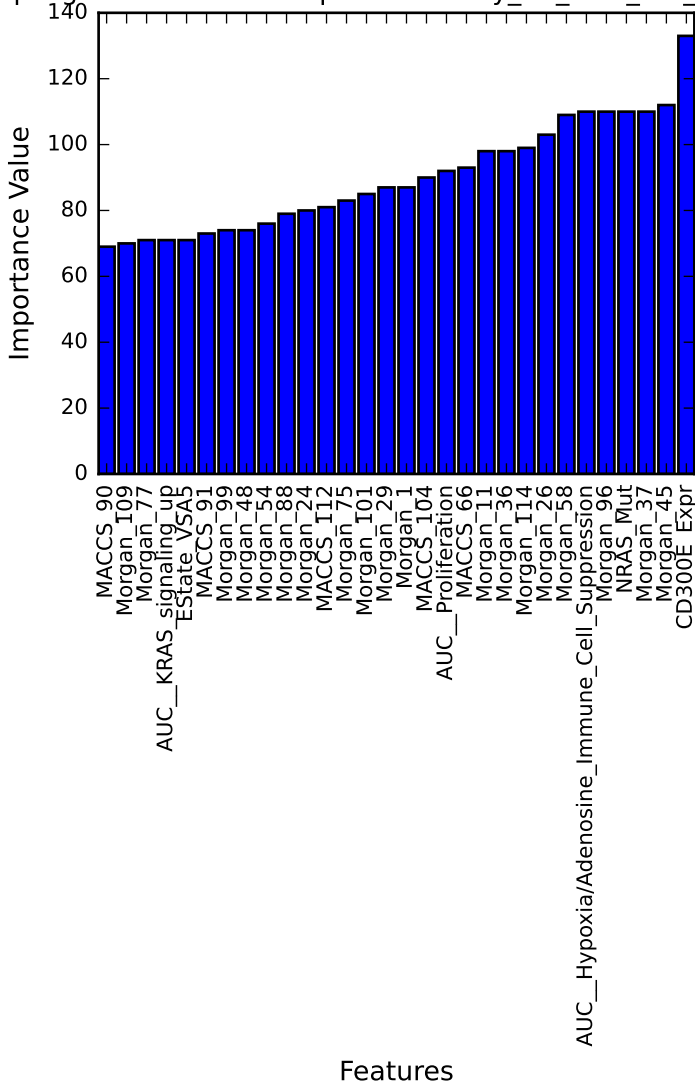
Top LightGBM Feature Importance Only_PC_Feat_Var_inhibitor
