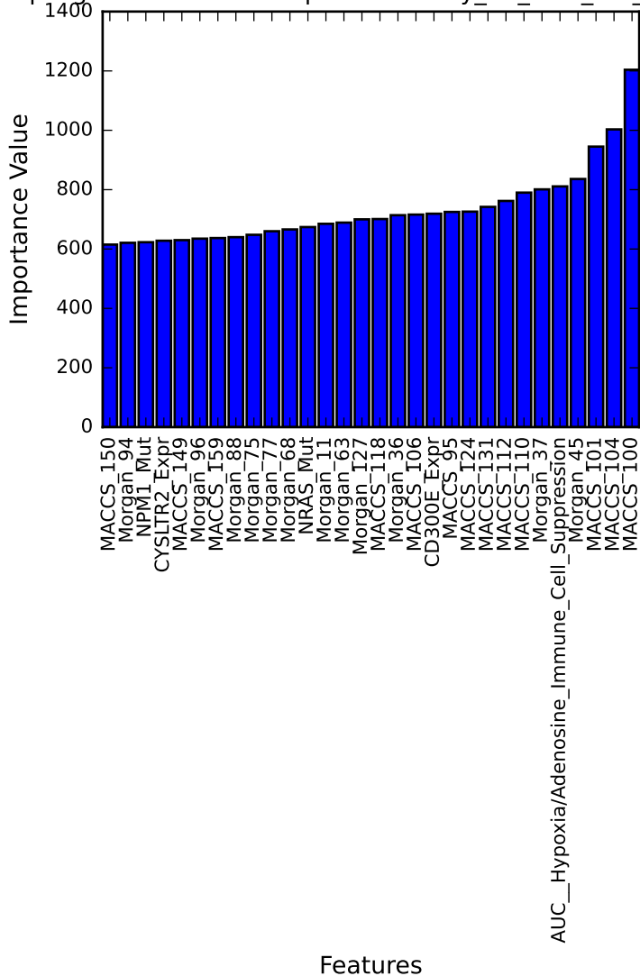
Top LightGBM Feature Importance Only_PC_Feat_Var_random
