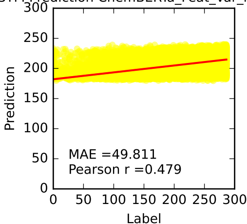
LSTM Prediction ChemBERTa_Feat_Var_inhibitor
