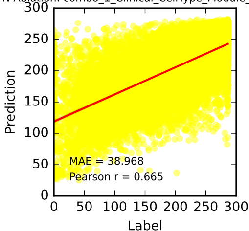
TabPFN Ablation: combo_1_Clinical_CellType_Module_Drug_Embed
