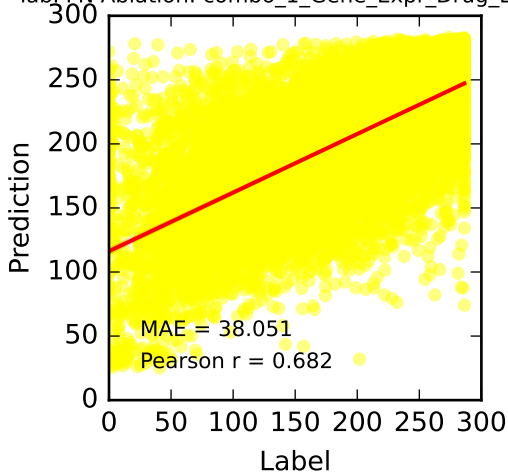
TabPFN Ablation: combo_1_Gene_Expr_Drug_Embed
