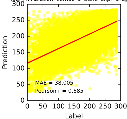
TabPFN Ablation: combo_1_Gene_Expr_Drug_PC
