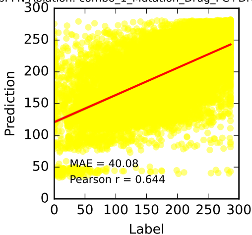
TabPFN Ablation: combo_1_Mutation_Drug_PC+Drug_Embed
