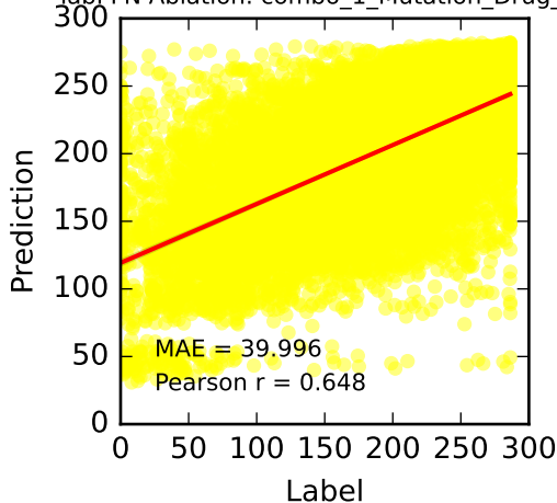
TabPFN Ablation: combo_1_Mutation_Drug_PC
