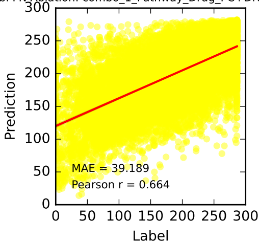
TabPFN Ablation: combo_1_Pathway_Drug_PC+Drug_Embed
