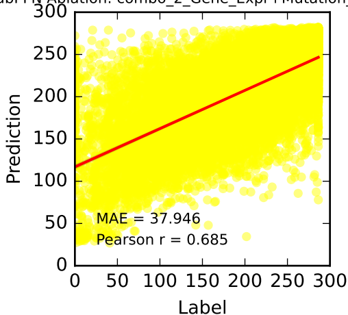
TabPFN Ablation: combo_2_Gene_Expr+Mutation_Drug_PC
