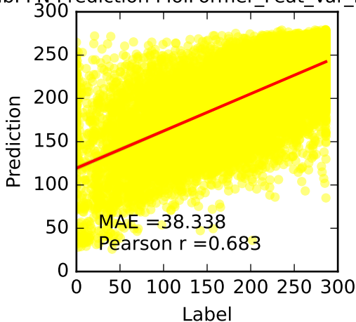
TabPFN Prediction MolFormer_Feat_Var_inhibitor
