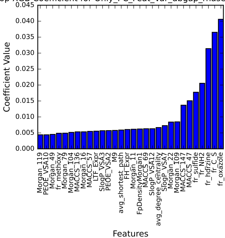
Top XGB Coefficient for Only_PC_Feat_Var_dbgap_rnaseq_sample
