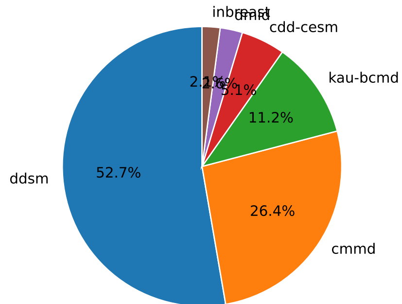
Pie chart
