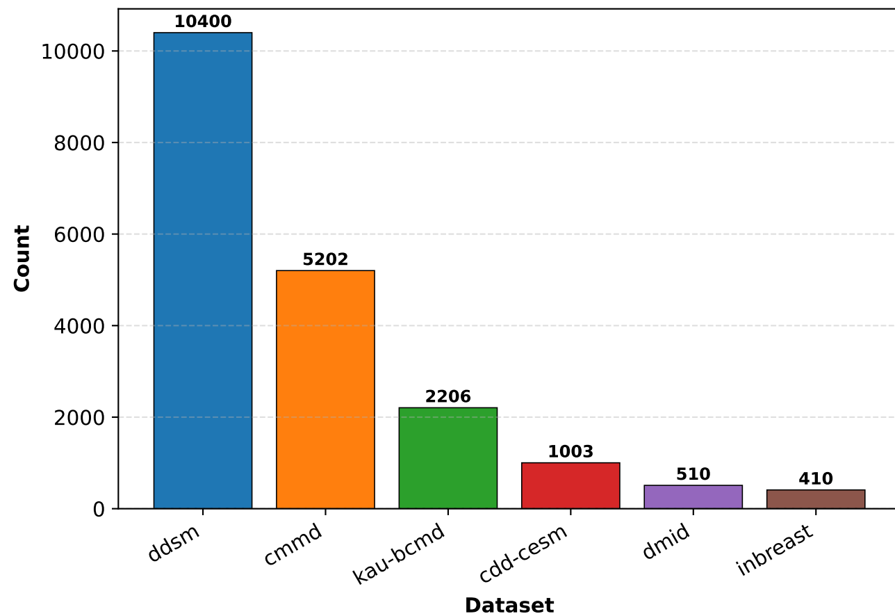
Bar chart
