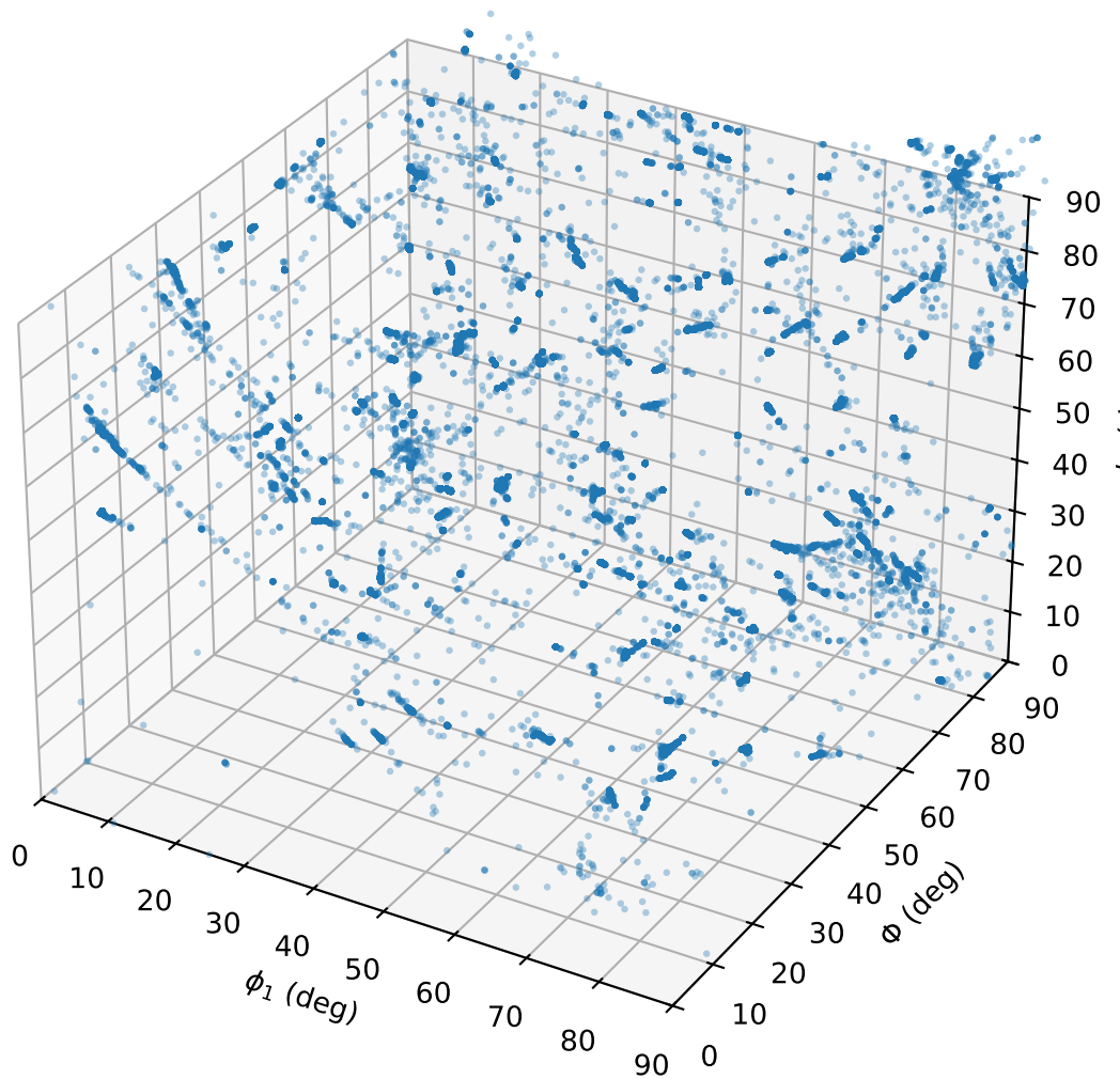
Euler cube scatter (cubic reduced \sim [0,90]^3 )
