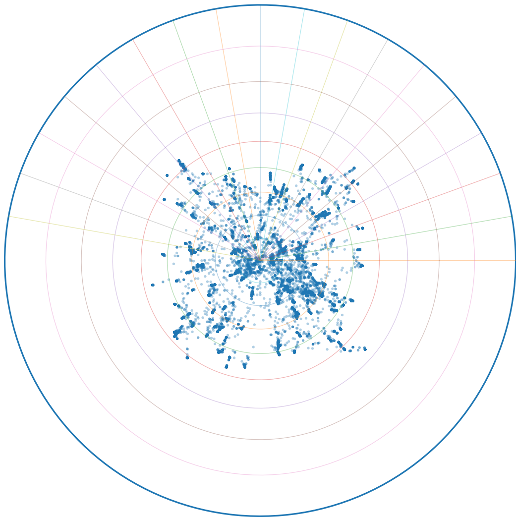
Stereogram: crystal [001] in sample (full net)
