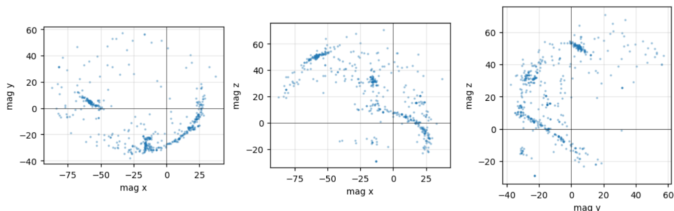
Magnetometer scatter — off-center, non-spherical = uncalibrated
