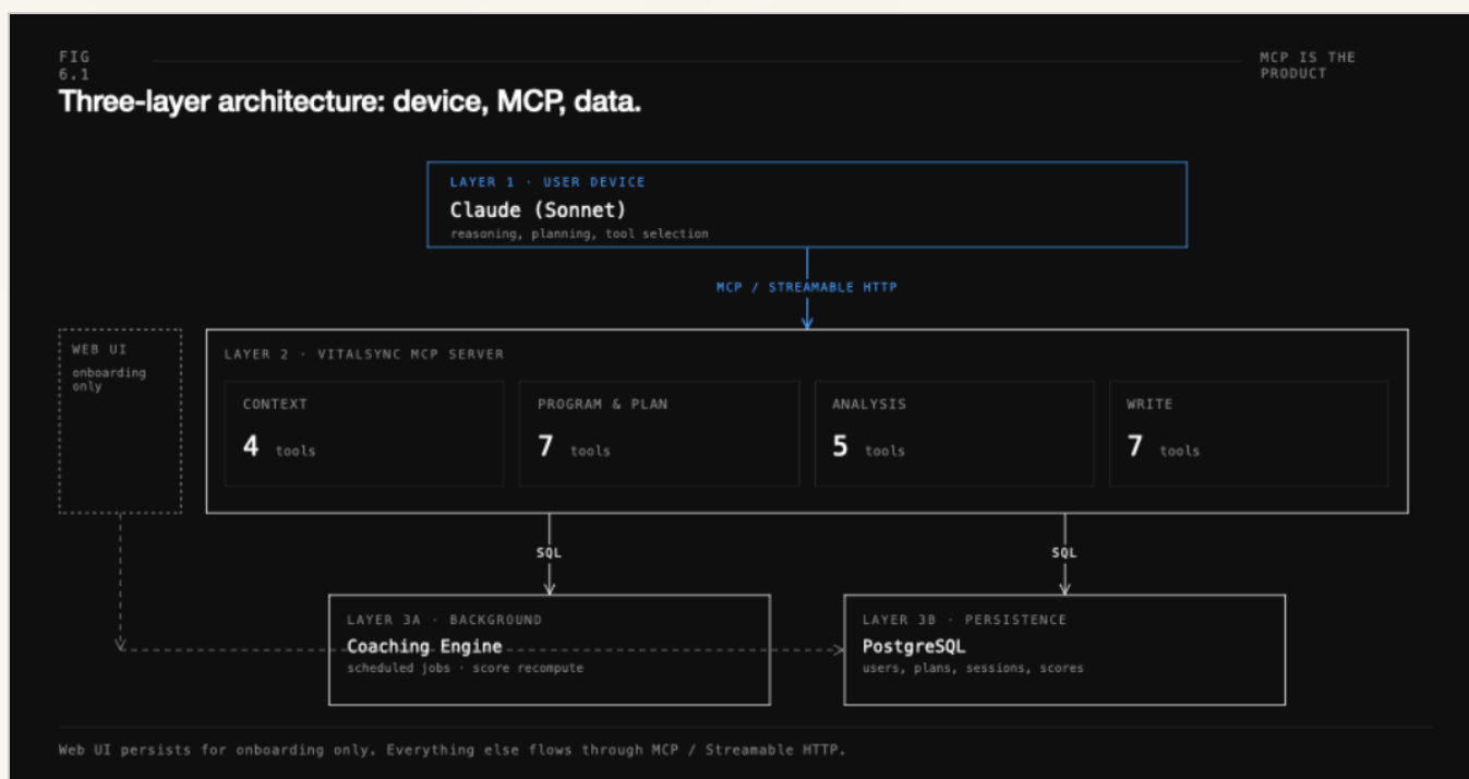
FIG 6.1 Final headless coach architecture — Claude, MCP server, coaching engine, database.
