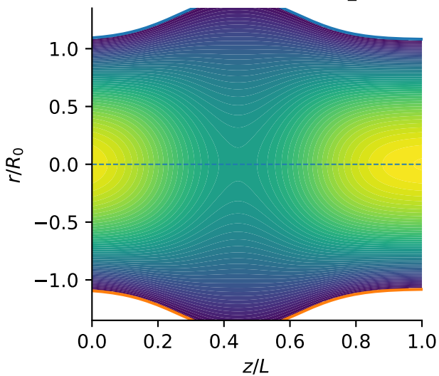
Sample 310 | expanded | newtonian
