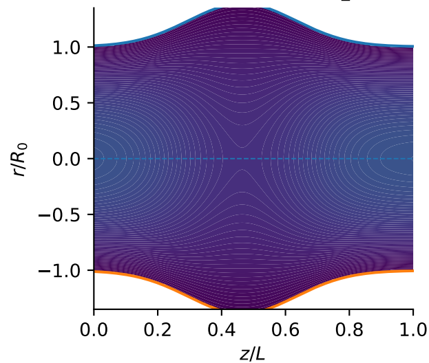
Sample 387 | expanded | newtonian
