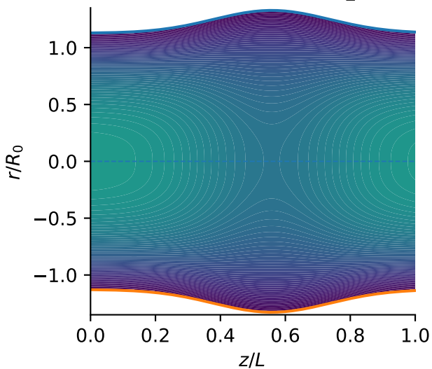
Sample 446 | sinusoidal | power_law
