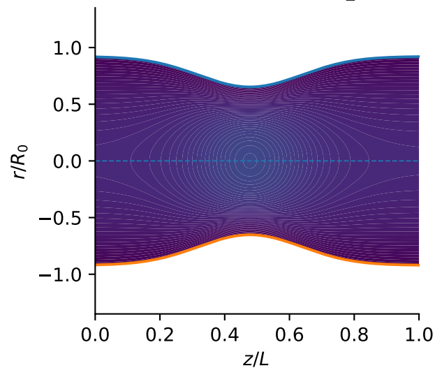
Sample 467 | sinusoidal | newtonian
