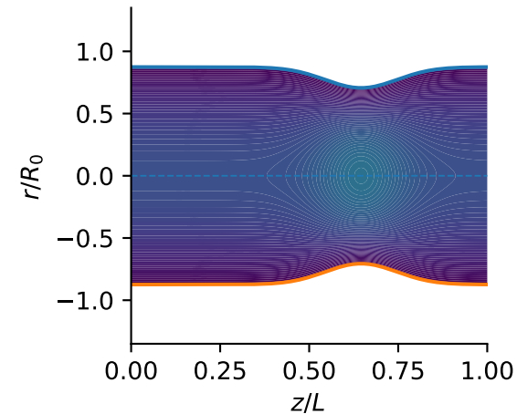
expanded | newtonian | sample 305 Delta P = 1.300e+00, Q = 6.582e-01, u_max = 3.701e-01
