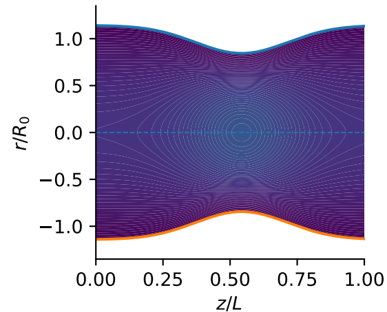
expanded | power_law | sample 395 Delta P = 1.586e+00, Q = 2.121e+00, u_max = 1.040e-01
