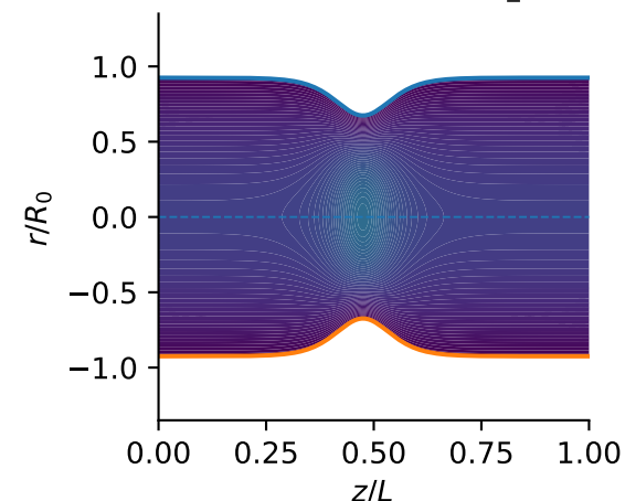
hyperbolic_constriction | newtonian | sample 40 Delta P = 1.286e+00, Q = 2.616e-01, u_max = 3.665e-01
