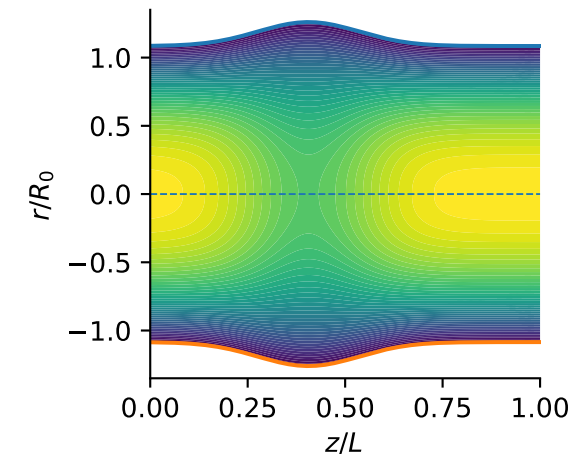
sinusoidal | power_law | sample 149 Delta P = 1.839e+00, Q = 7.946e-01, u_max = 8.191e-01
