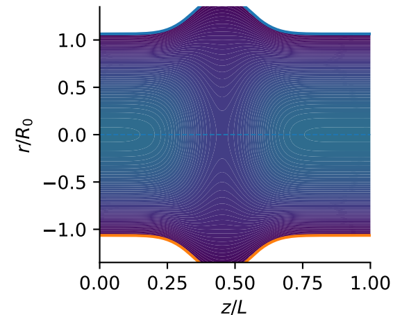
sinusoidal | newtonian | sample 430 Delta P = 1.409e+00, Q = 1.180e+00, u_max = 8.247e-01
