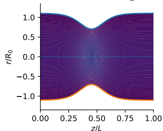
hyperbolic_constriction | power_law | sample 139 Delta P = 7.419e-01, Q = 1.612e-01, u_max = 1.880e-01
