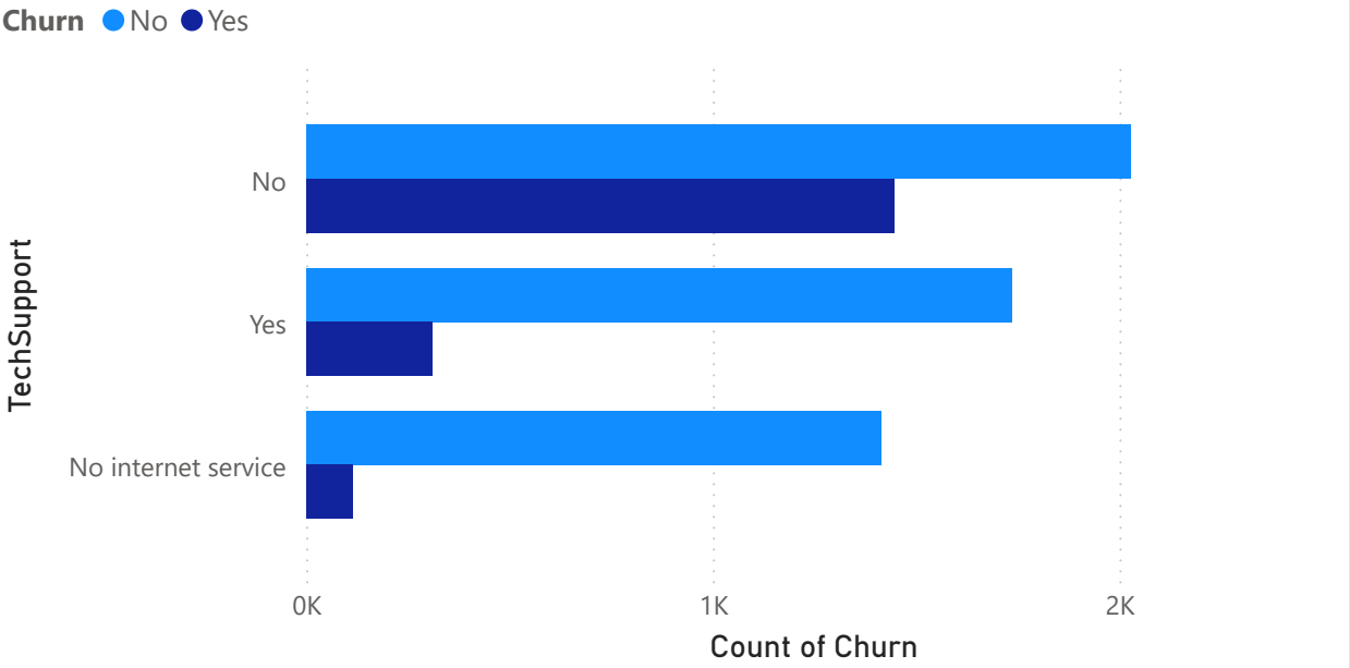
Count of Churn by TechSupport and Churn
