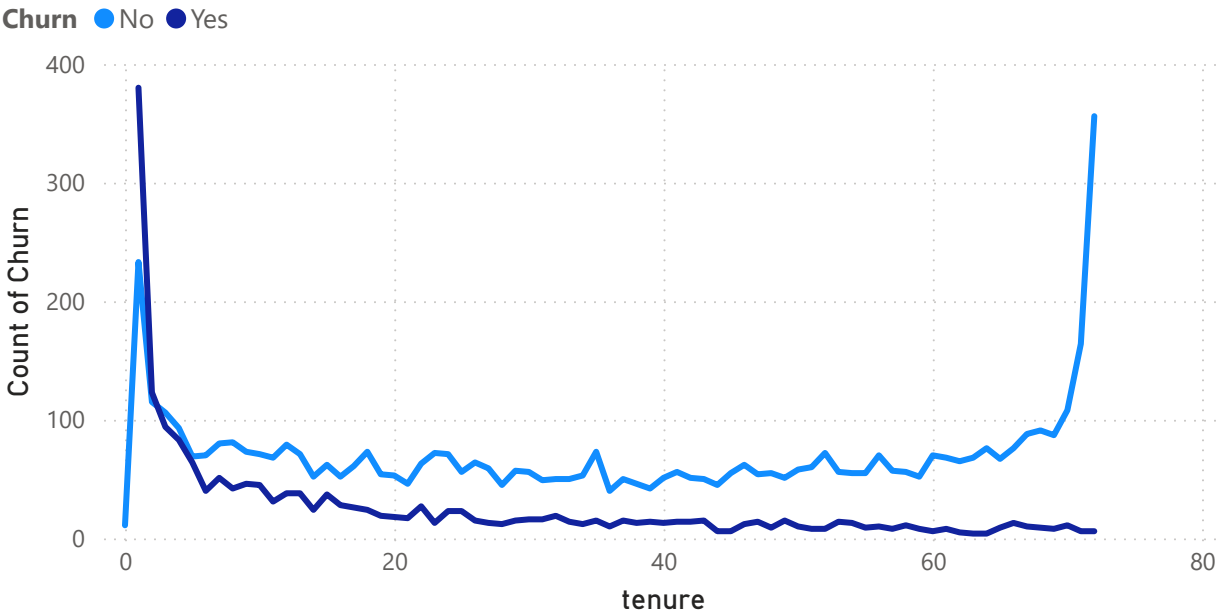
Count of Churn by tenure and Churn
