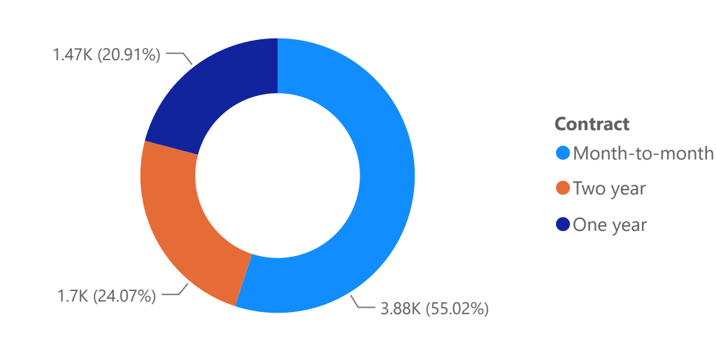
Count of Churn by Contract
