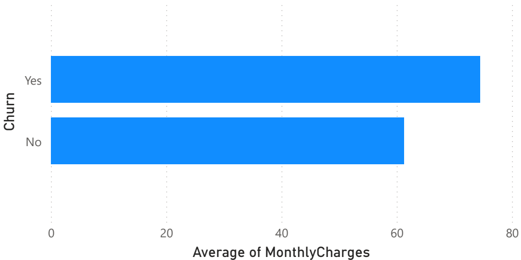
Average of MonthlyCharges by Churn
