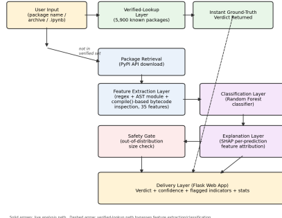
Figure 1: PyPIGuard architecture. Solid arrows: live analysis path. Dashed arrow: verified-lookup shortcut.
