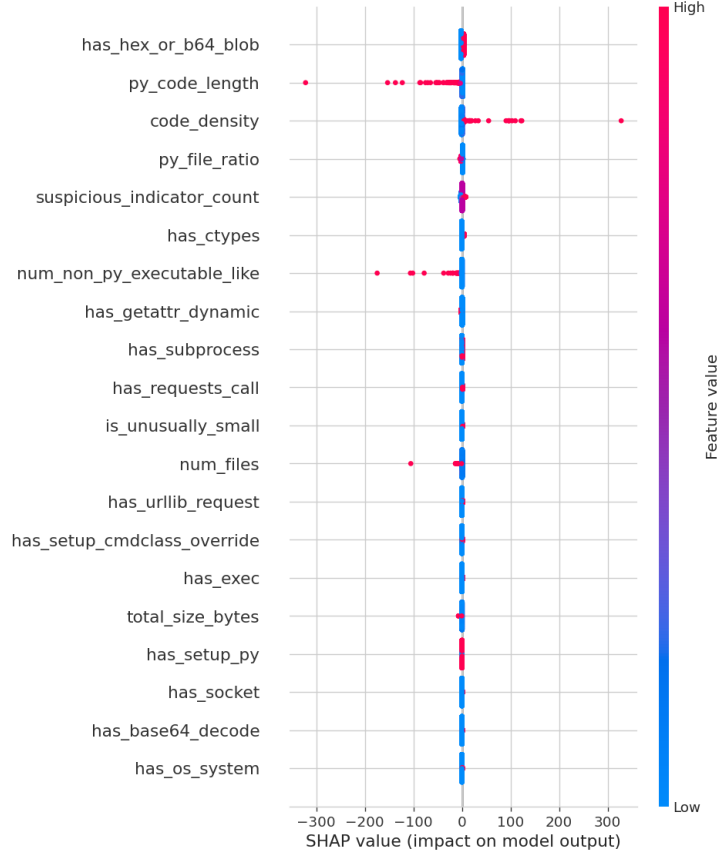
Figure 2: SHAP global feature-importance summary, illustrating the explainability layer.
