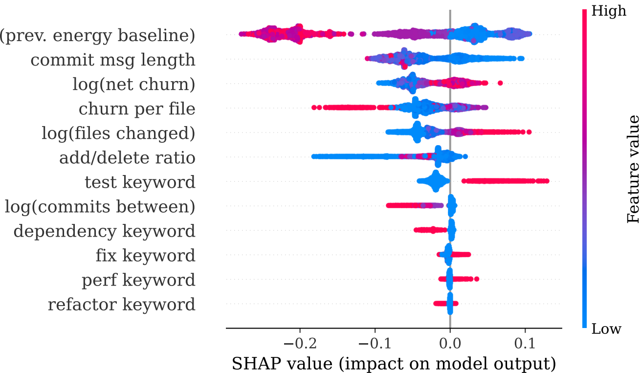
SHAP feature importance for energy-regression prediction
