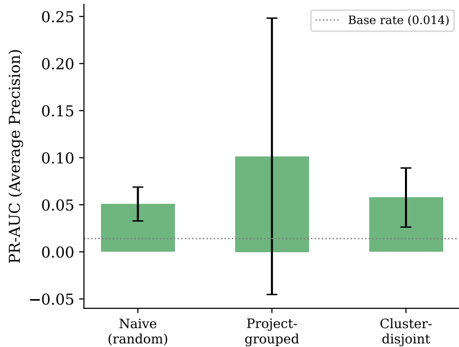
(b) PR-AUC by evaluation protocol
