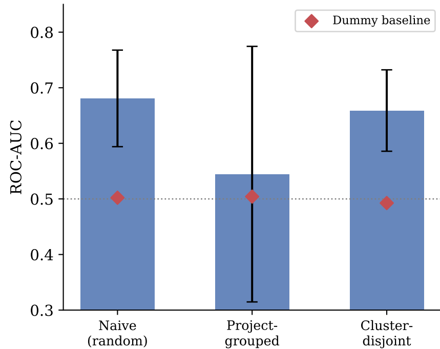
(a) ROC-AUC by evaluation protocol
