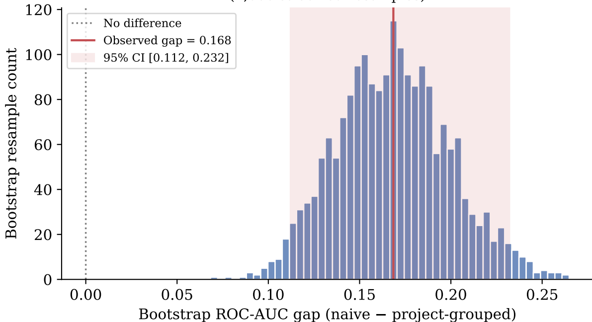
Bootstrap distribution of the naive-vs-grouped AUC gap (2,000 stratified resamples)
