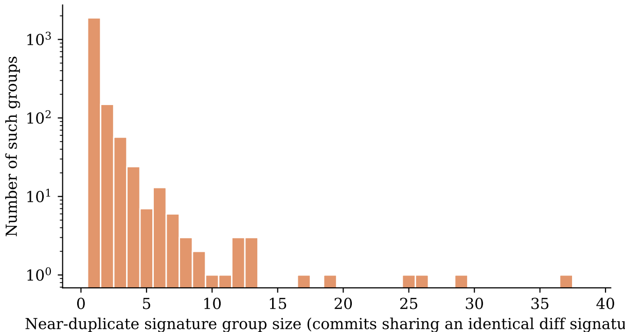
Near-duplicate diff signatures across the dataset (48.9% of all transitions belong to a group of size > 1 )
