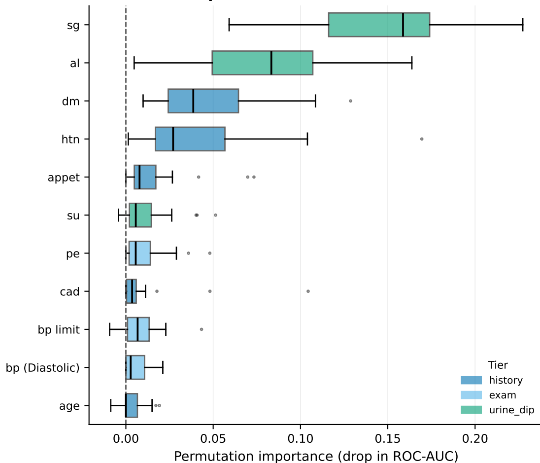
A. Importance across 25 outer folds
