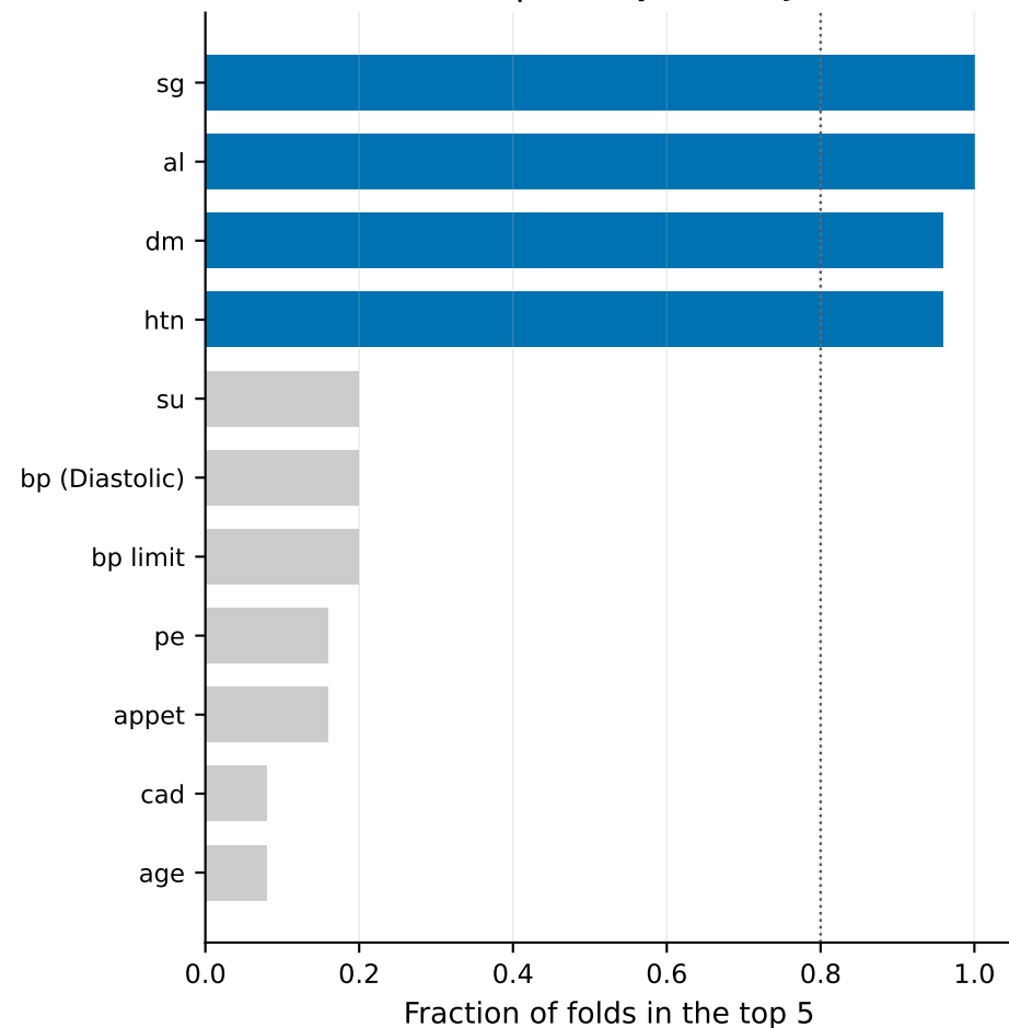
B. Top-5 selection frequency Kendall's W = 0.694 | mean pairwise Jaccard = 0.674
