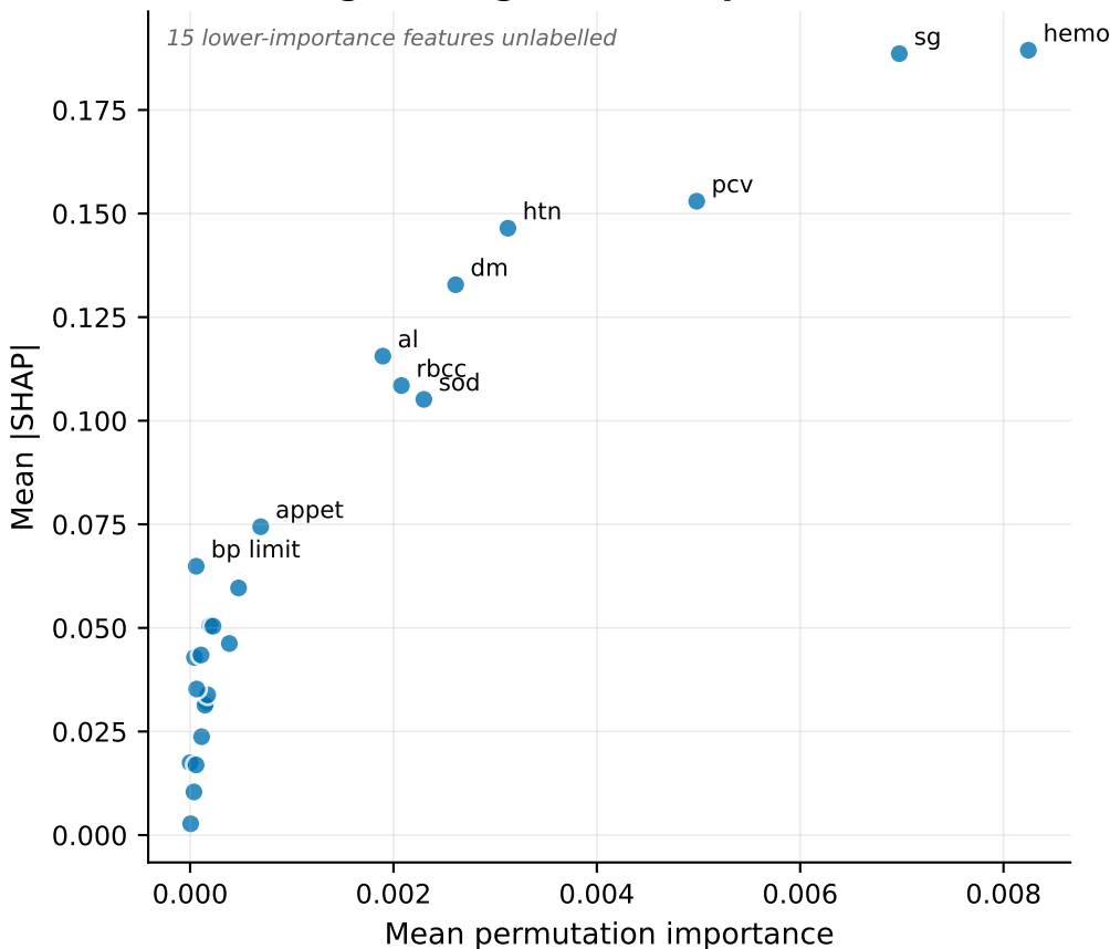
Figure R11. SHAP vs permutation importance Full valid (Logistic regression), Spearman rho = 0.905
