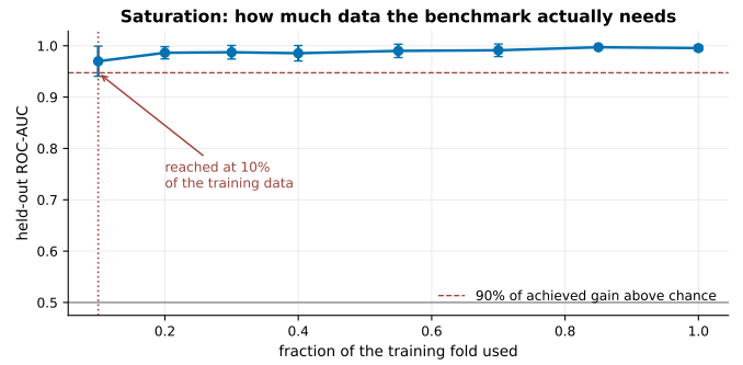
Fig. 6. Held-out discrimination against the fraction of the training fold used. Performance approached its observed plateau with approximately 10% of each training fold, so the benchmark provides little practical headroom for distinguishing the evaluated methods by sample efficiency under this design.
