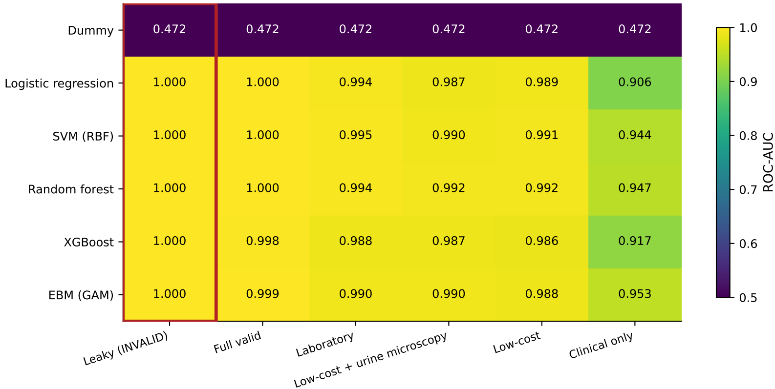
Figure R1. Nested-CV ROC-AUC by model and feature configuration (uncalibrated; pooled out-of-fold predictions)
