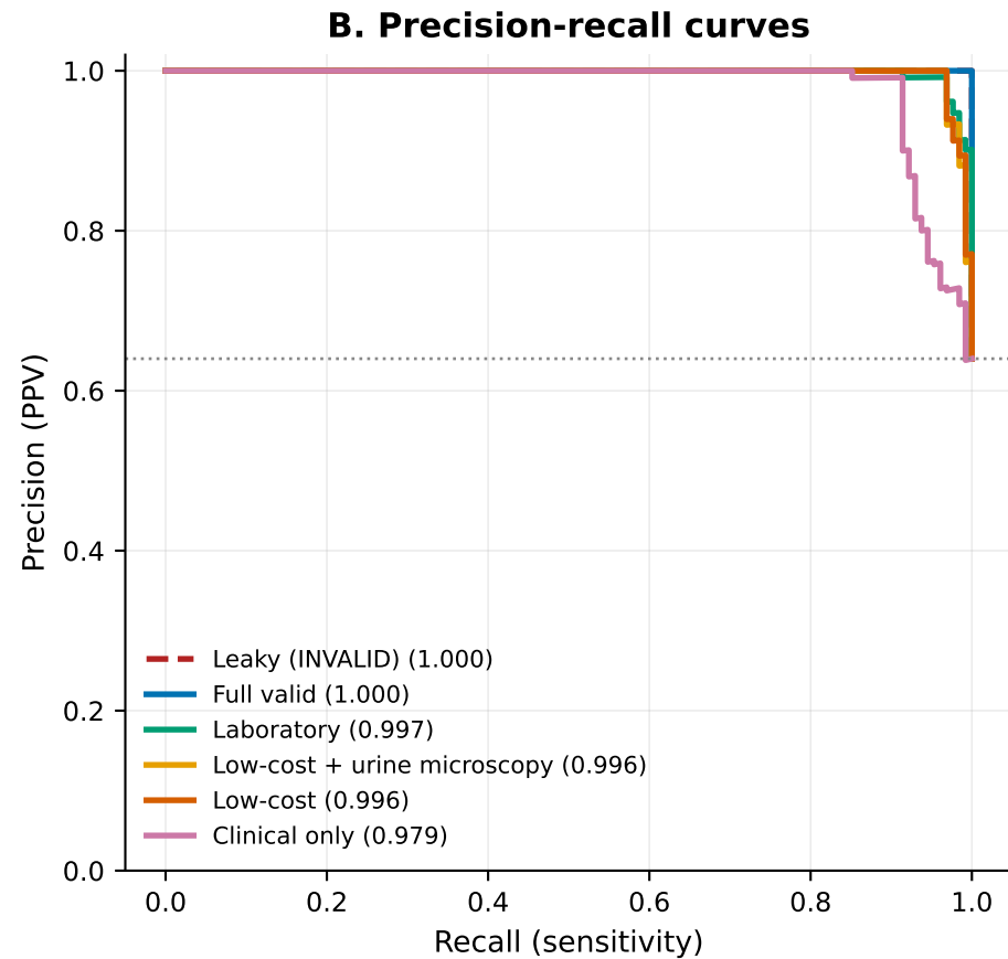
Figure R4. Discrimination, pooled out-of-fold predictions
