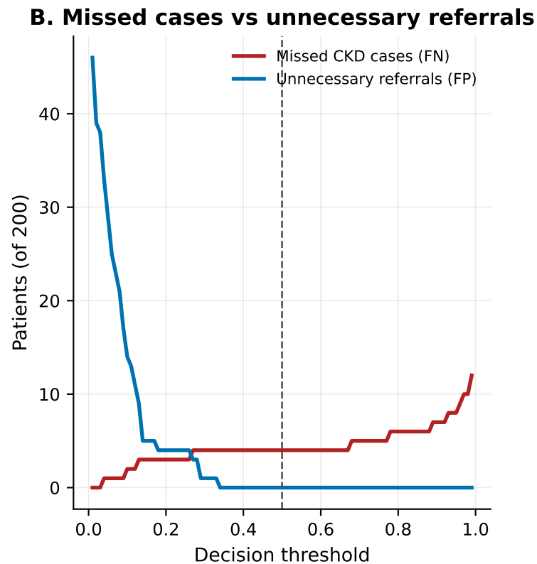
Figure R7. Screening trade-offs, low-cost model (SVM (RBF), Isotonic)
