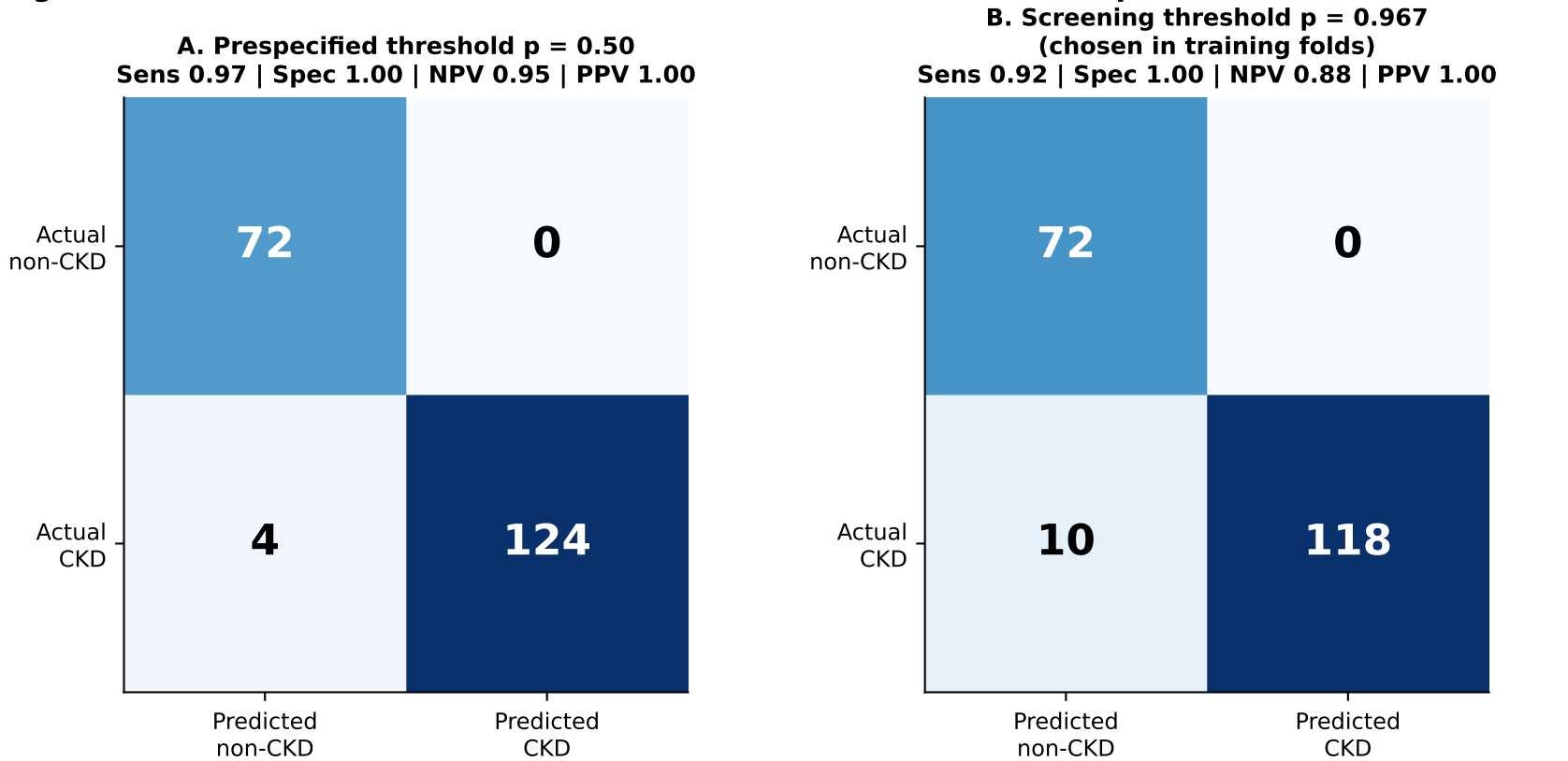
Figure R8. Low-cost model confusion matrices (SVM (RBF), Isotonic, pooled out-of-fold, n = 200)
