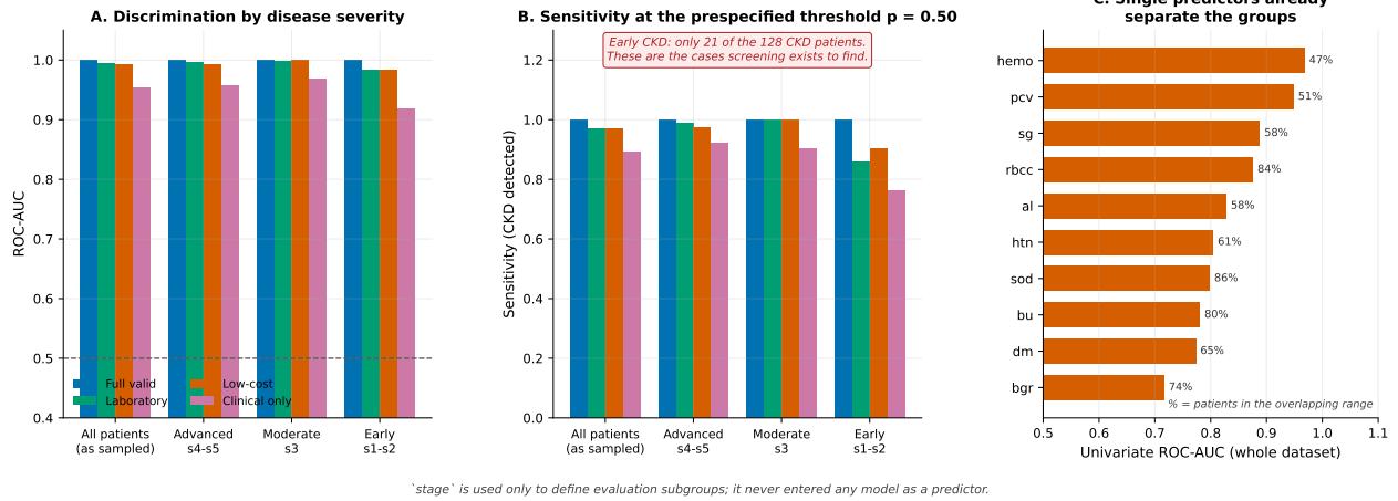
Fig. 1. Performance by disease-stage subgroup. Discrimination measured on the sample as a whole is systematically optimistic relative to the early-stage patients that screening exists to find. Panel C shows that single predictors already separate the groups, which is why no multivariable learning is required to reach the ceiling.
