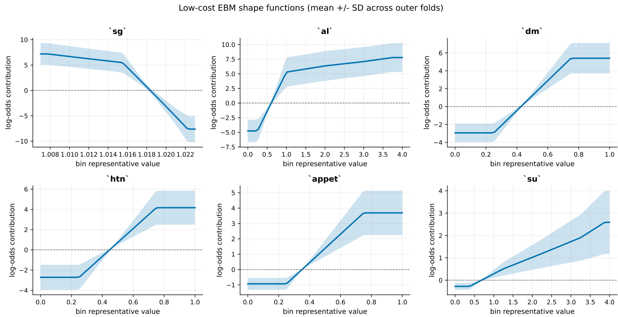
Fig. 4. Fitted shape functions of the low-cost additive model, averaged over 25 outer folds (shaded band: \pm 1 SD). Directions are clinically coherent: low urine specific gravity raises risk, albuminuria raises it steeply, and diabetes, hypertension and poor appetite all push the same way.
