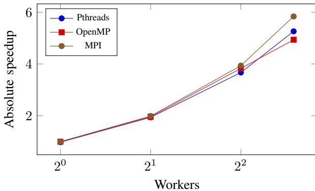
Fig. 2. Absolute speedup vs. worker count on hickory, large dataset.
