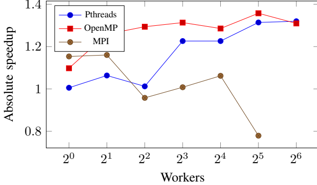
Fig. 1. Absolute speedup vs. worker count on maple, medium dataset.
