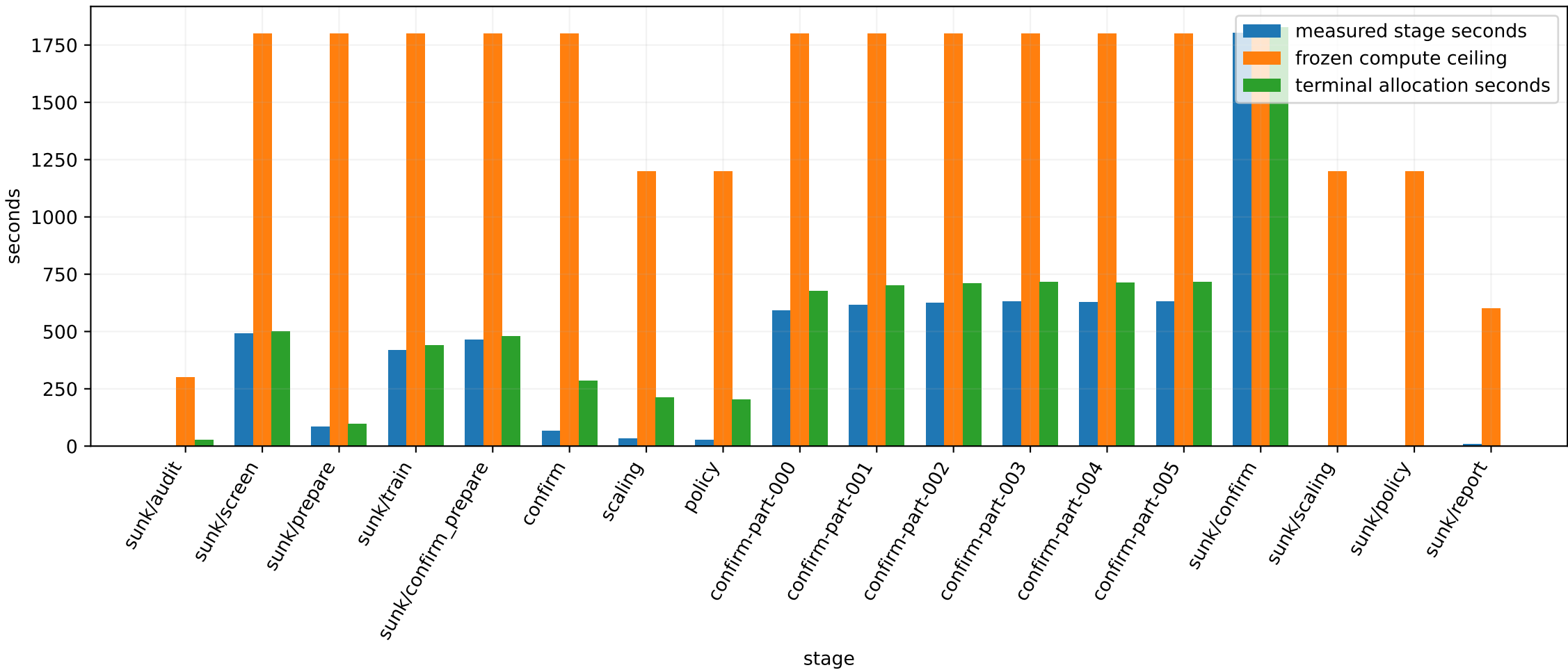
Stage compute and frozen budgets
