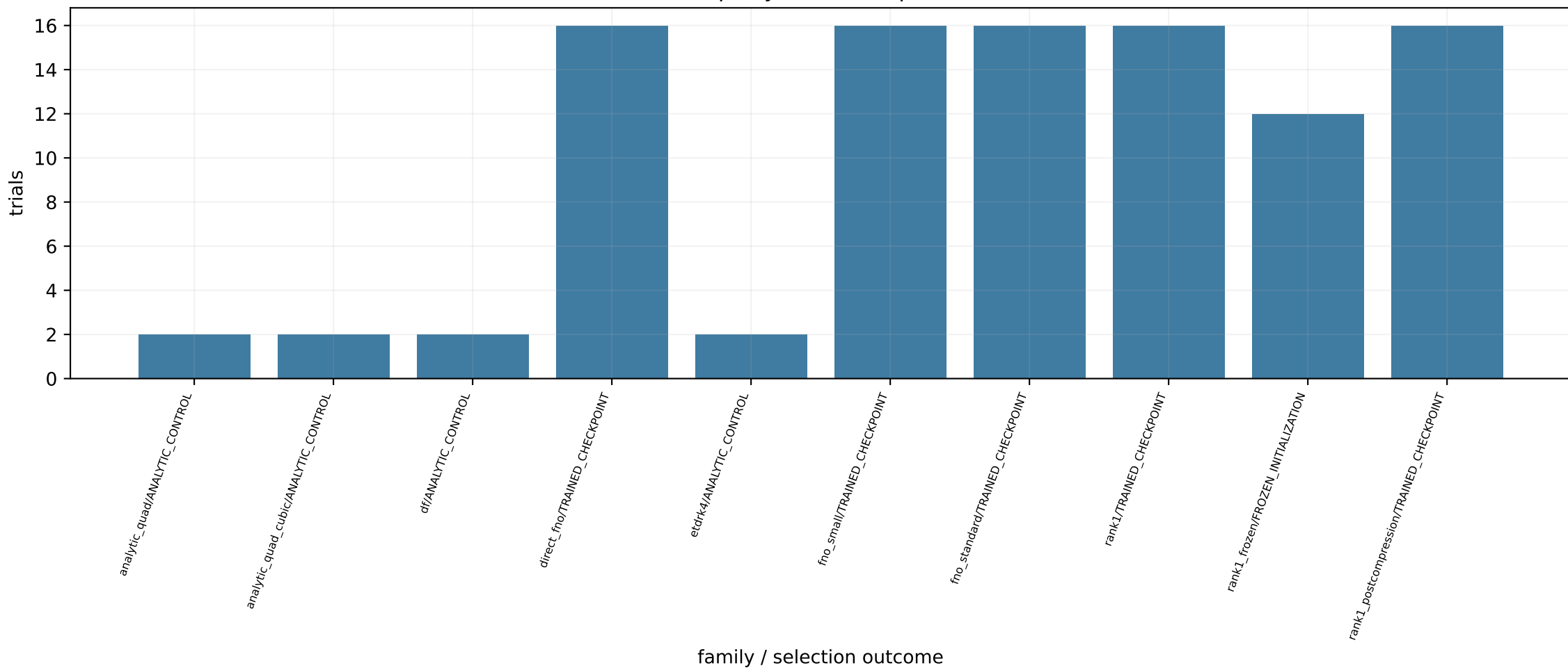
Baseline adequacy and checkpoint selections
