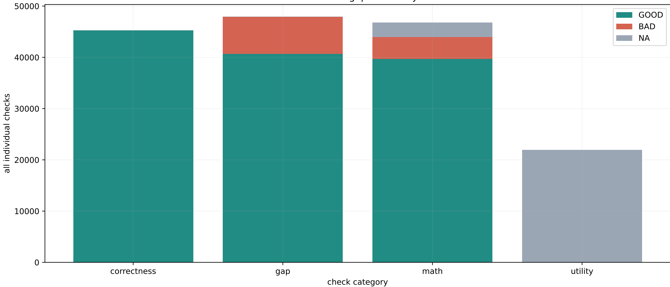
Correctness math gap and utility checks
