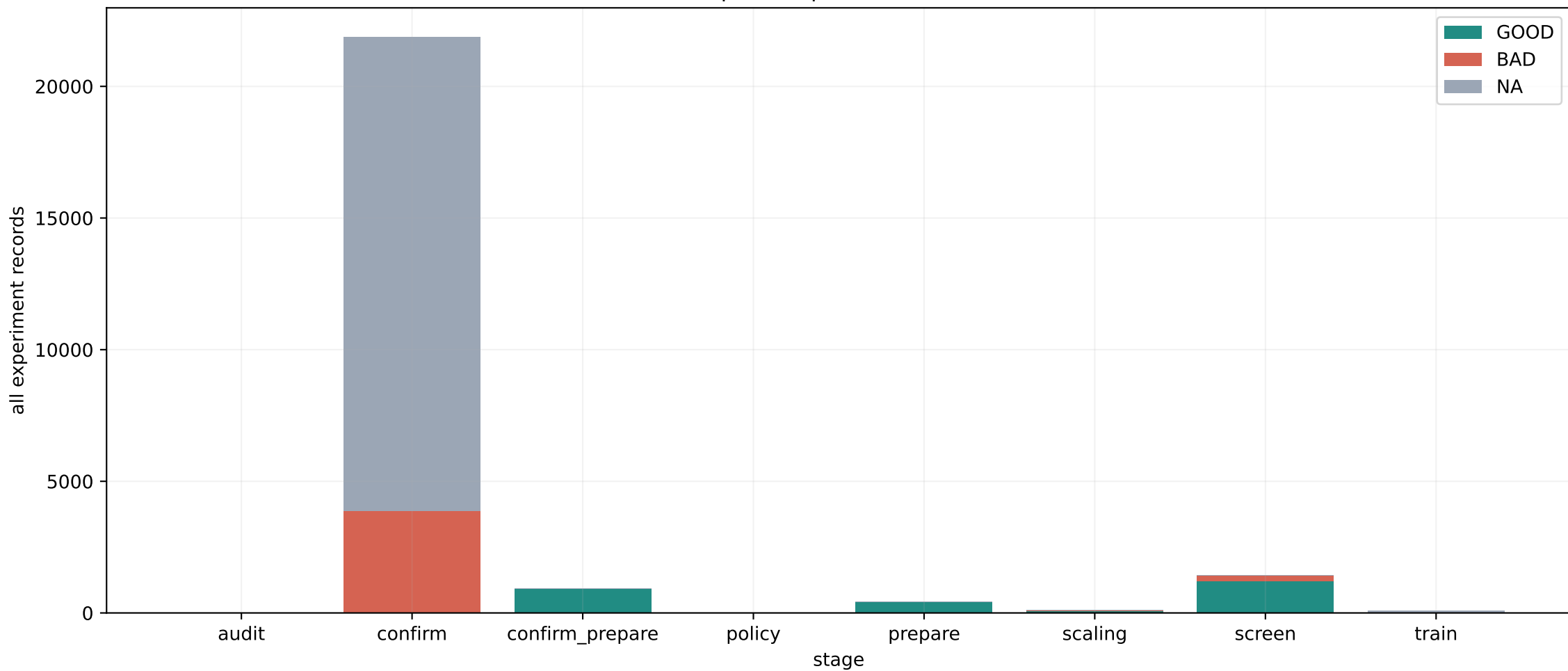
Complete experiment verdicts
