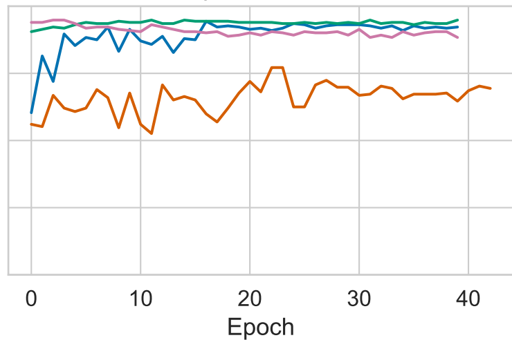
pretrained
