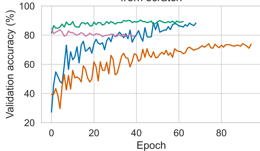
from scratch
