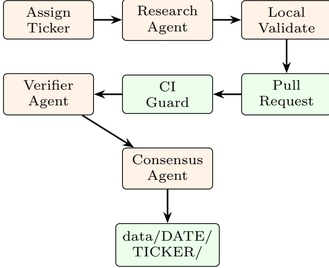
Figure 1: Distributed ingestion pipeline. Each contributor machine runs assignment, research, and validation locally; GitHub CI and peer agents provide trust anchors.
