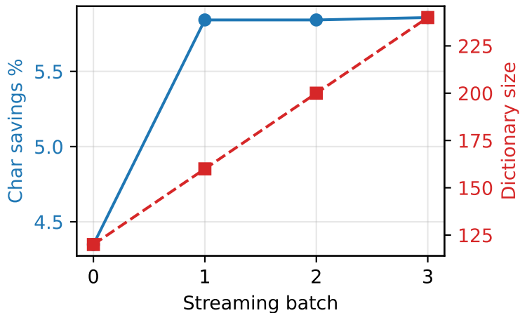
Dictionary learning curve (streaming, token-aware)
