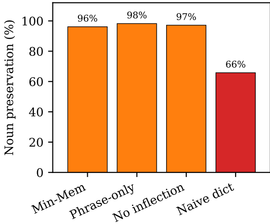
(b) Entity safety (noun tags)
