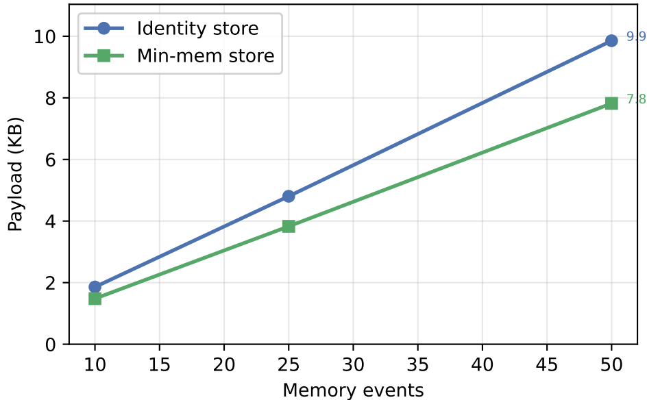
Storage growth: identity vs min-mem
