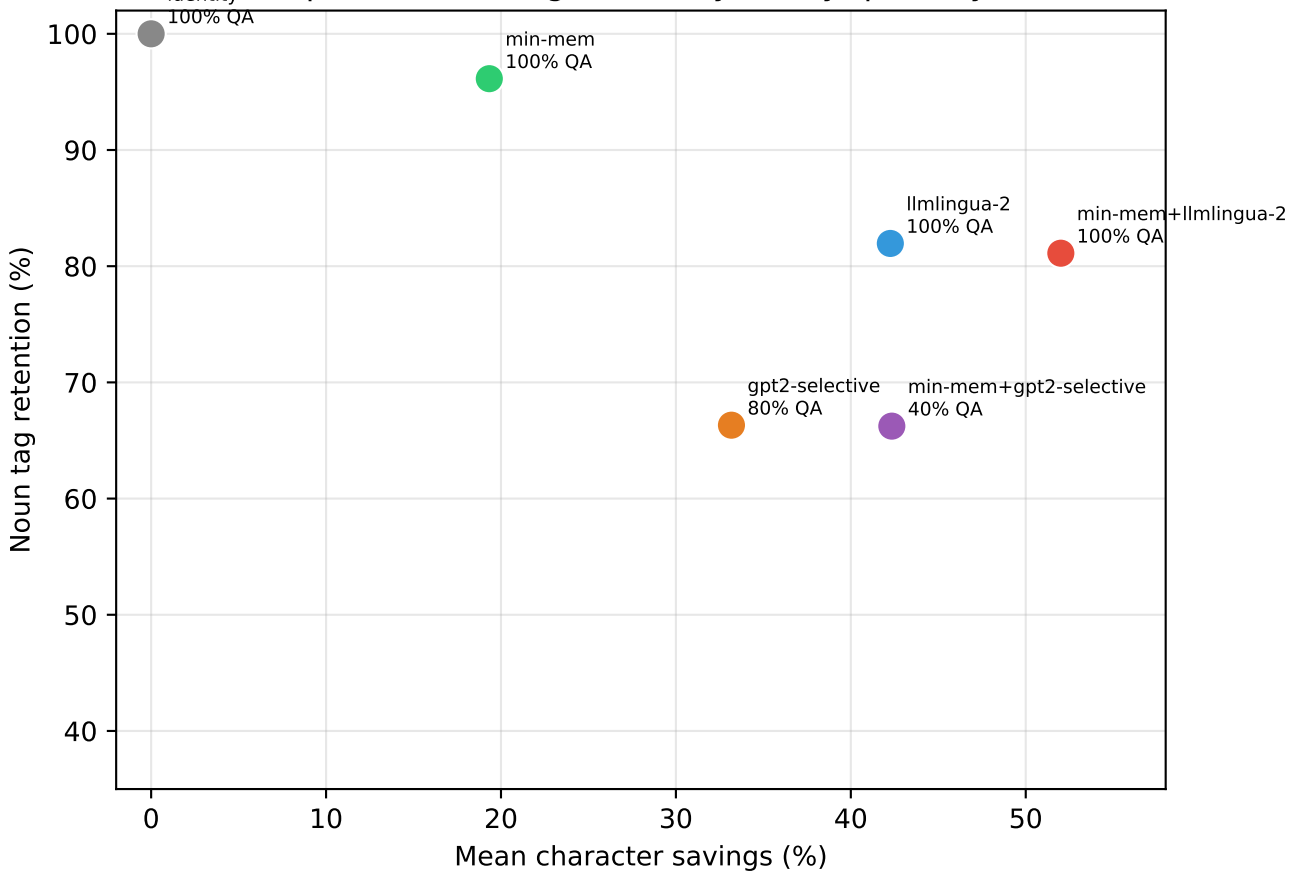
Tiered compression: savings vs entity safety (primary rate=0.5)
