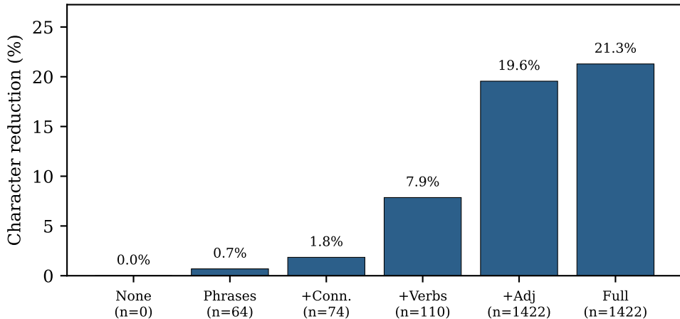
Dictionary ablation: savings vs dictionary size
