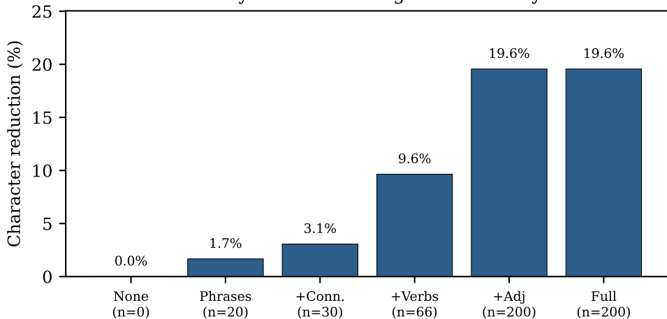
Dictionary ablation: savings vs dictionary size
