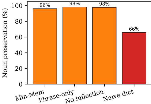
(b) Entity safety (noun tags)
