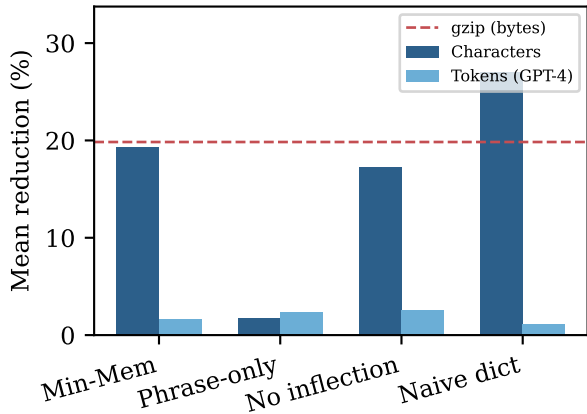
(a) Size reduction by method
