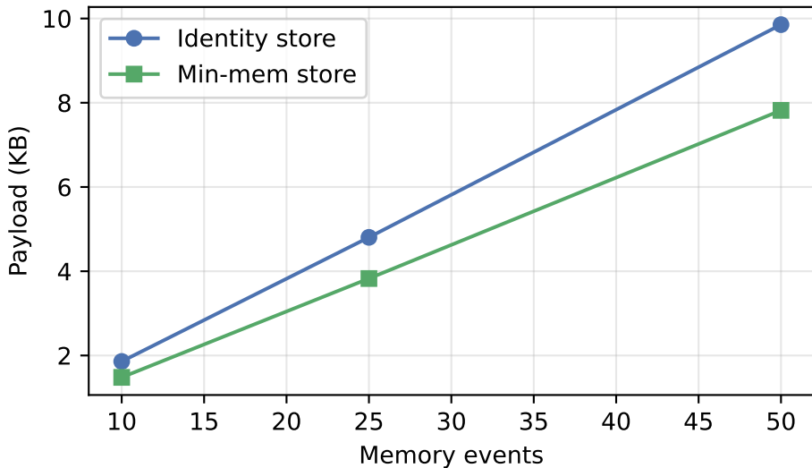
Memory growth: identity vs min-mem
