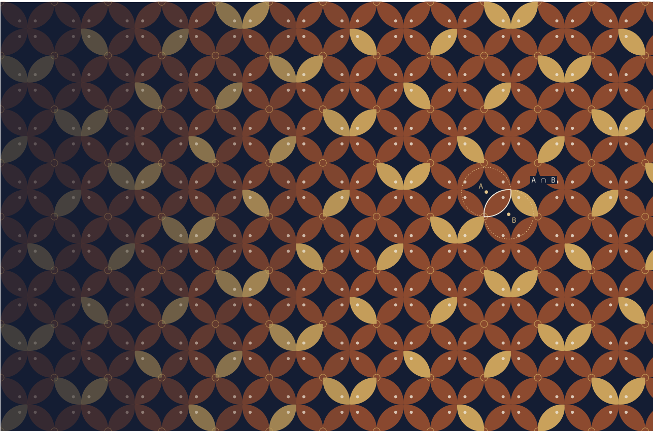
PLATE II KAWUNG, CONSTRUCTED Every petal of the Javanese kawung motif is the intersection of two circles, A \cap B : the set-theoretic reading of cultural form that runs through her work on ethnomathematics.
